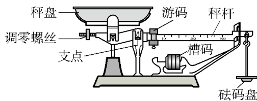
图6.1-7 案秤
